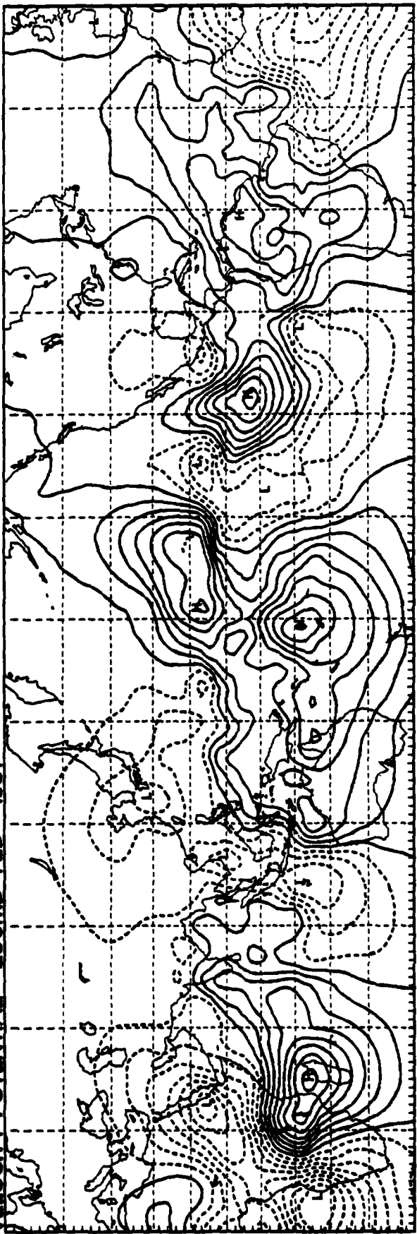
VELOCITY POTENTIAL 200MB FEB 1981
